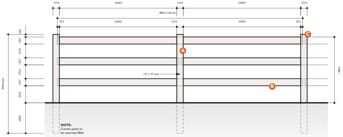
FENCE ELEVATION
